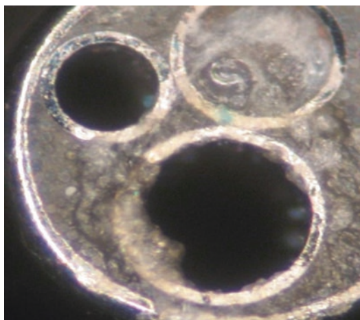
Fig. 5.8 View of salivary scope tip that was damaged by laser use. This changed the scope optics and deformed the working channel
